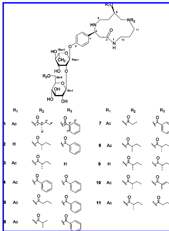
Figure 1. Structures of 1–11.
