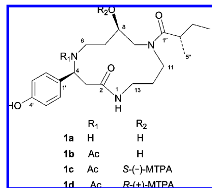
Figure 3. Structures of 1a–1d .
